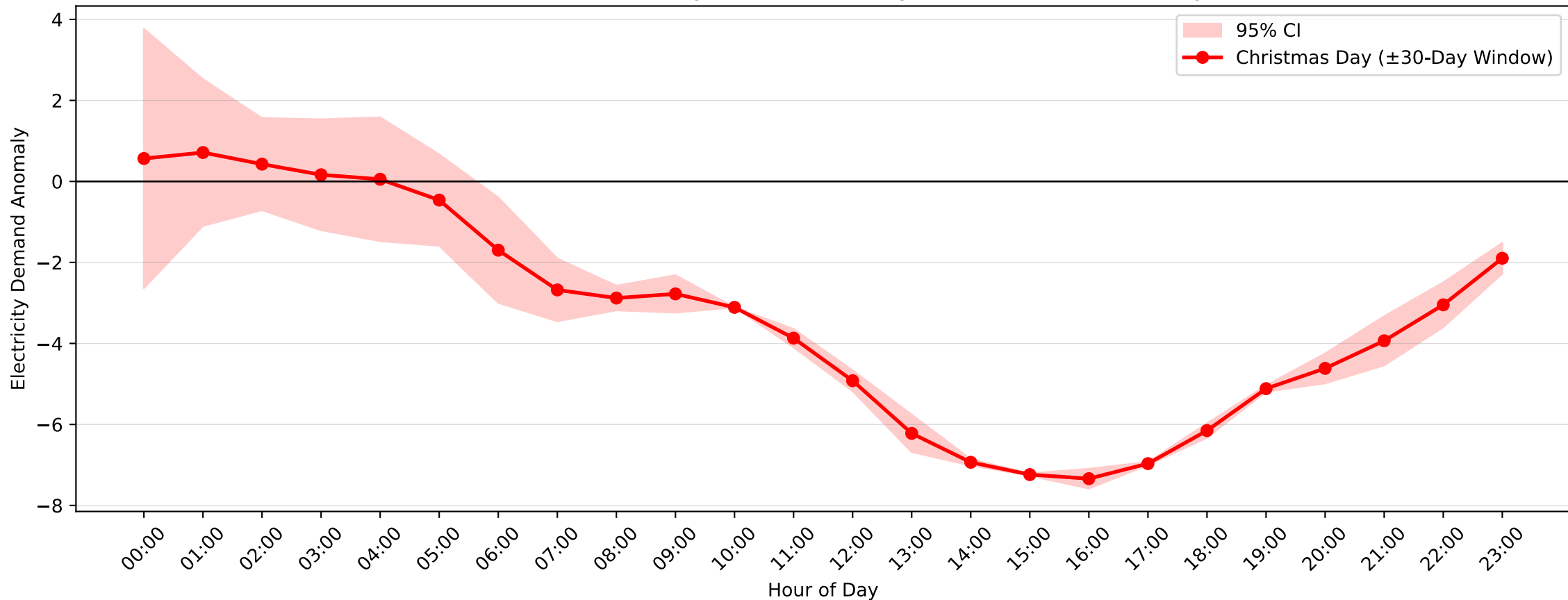
Hunters Hill Demand Anomaly: Christmas Day (2012–2013, \pm 30 -Day Window)
