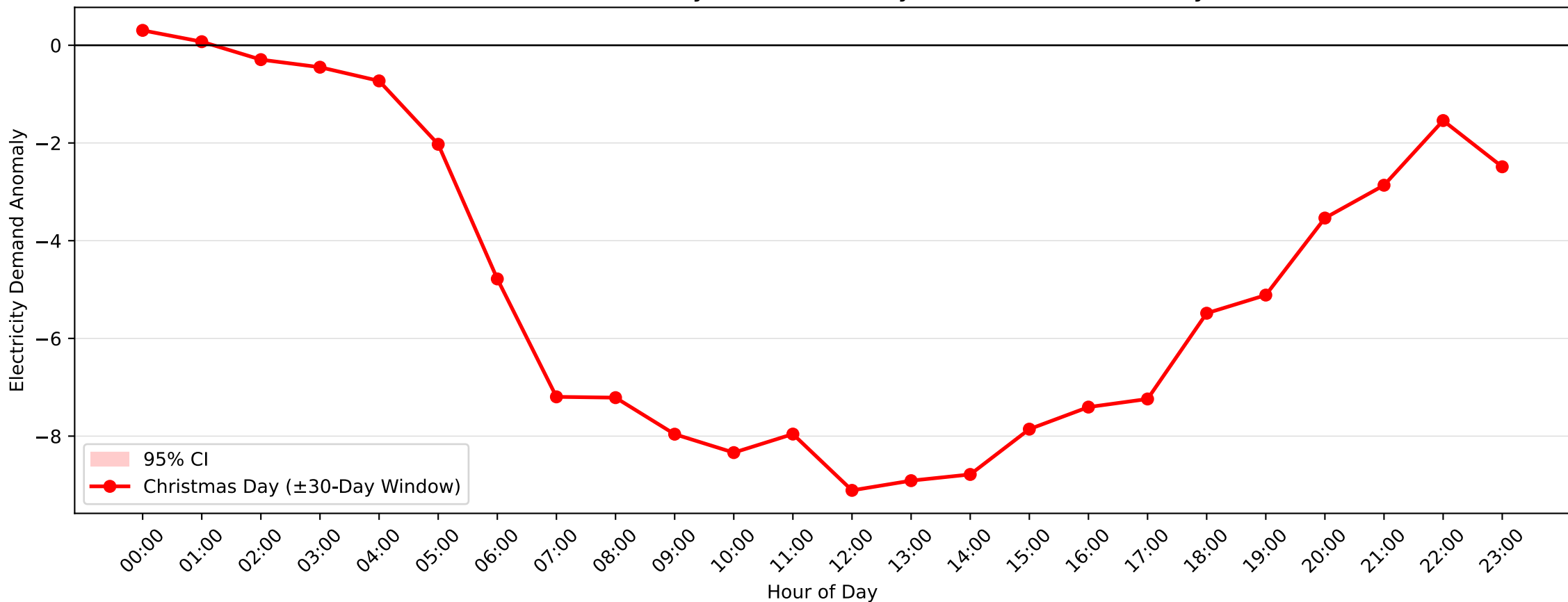
Hunters Hill Demand Anomaly: Christmas Day (2004–2005, \pm 30 -Day Window)
