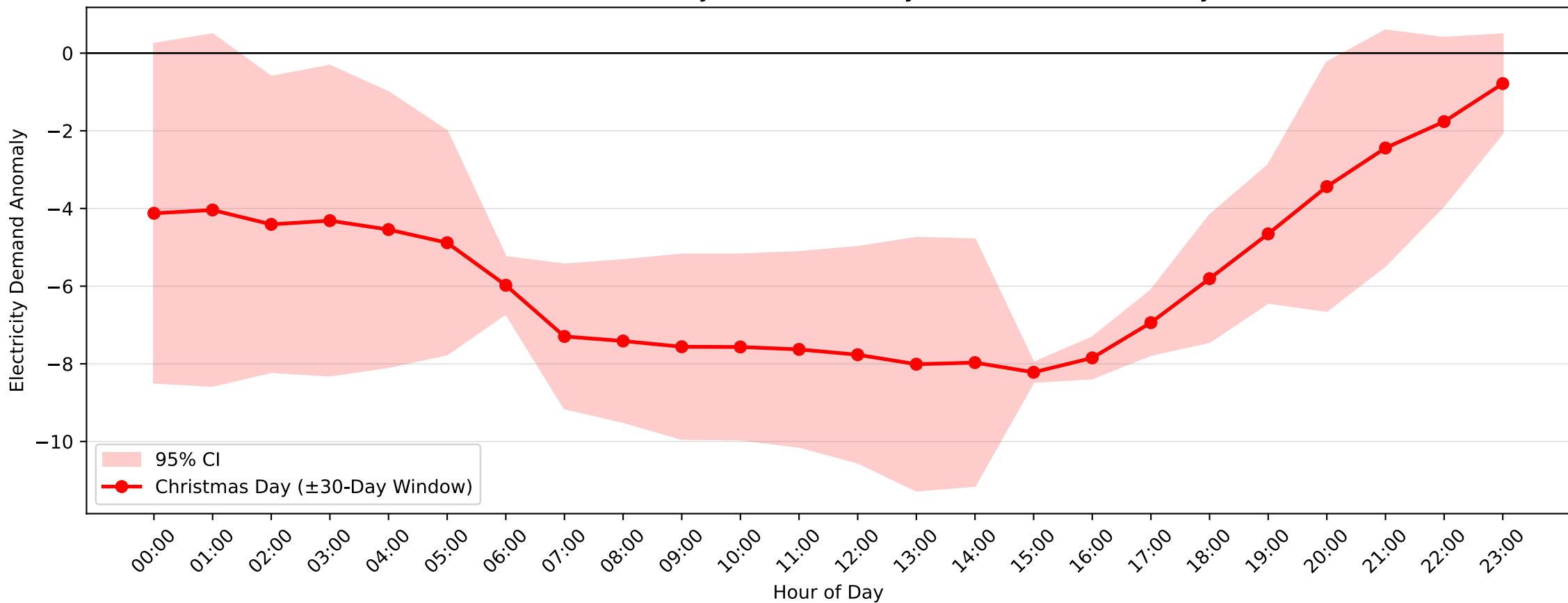
Hunters Hill Demand Anomaly: Christmas Day (2009-2010, \pm 30 -Day Window)
