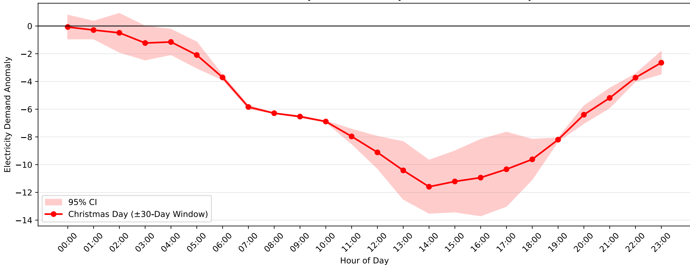
Hunters Hill Demand Anomaly: Christmas Day (2007-2008, \pm 30 -Day Window)
