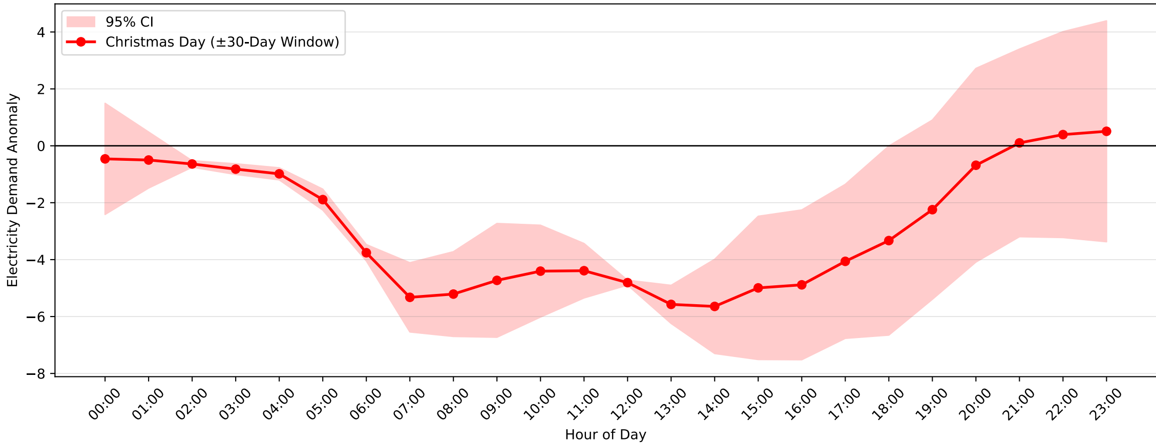
Hunters Hill Demand Anomaly: Christmas Day (2010-2011, \pm 30 -Day Window)
