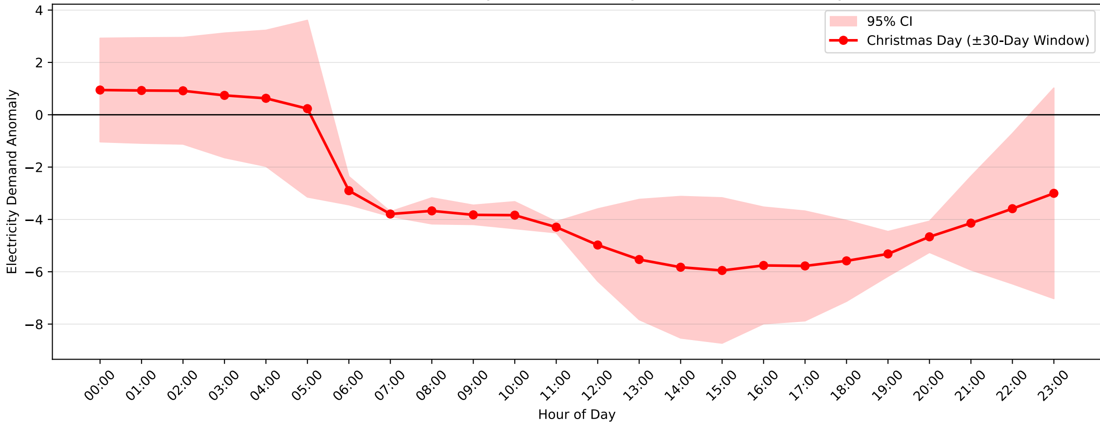
Hunters Hill Demand Anomaly: Christmas Day (2014–2015, \pm 30 -Day Window)
