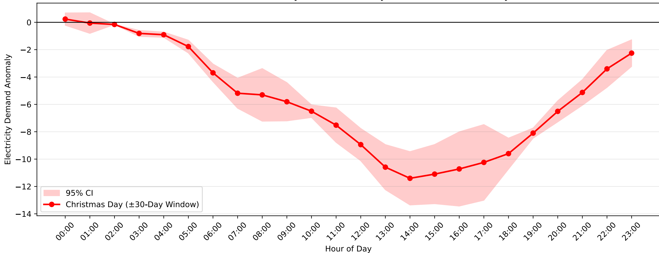
Hunters Hill Demand Anomaly: Christmas Day (2006–2007, \pm 30 -Day Window)
