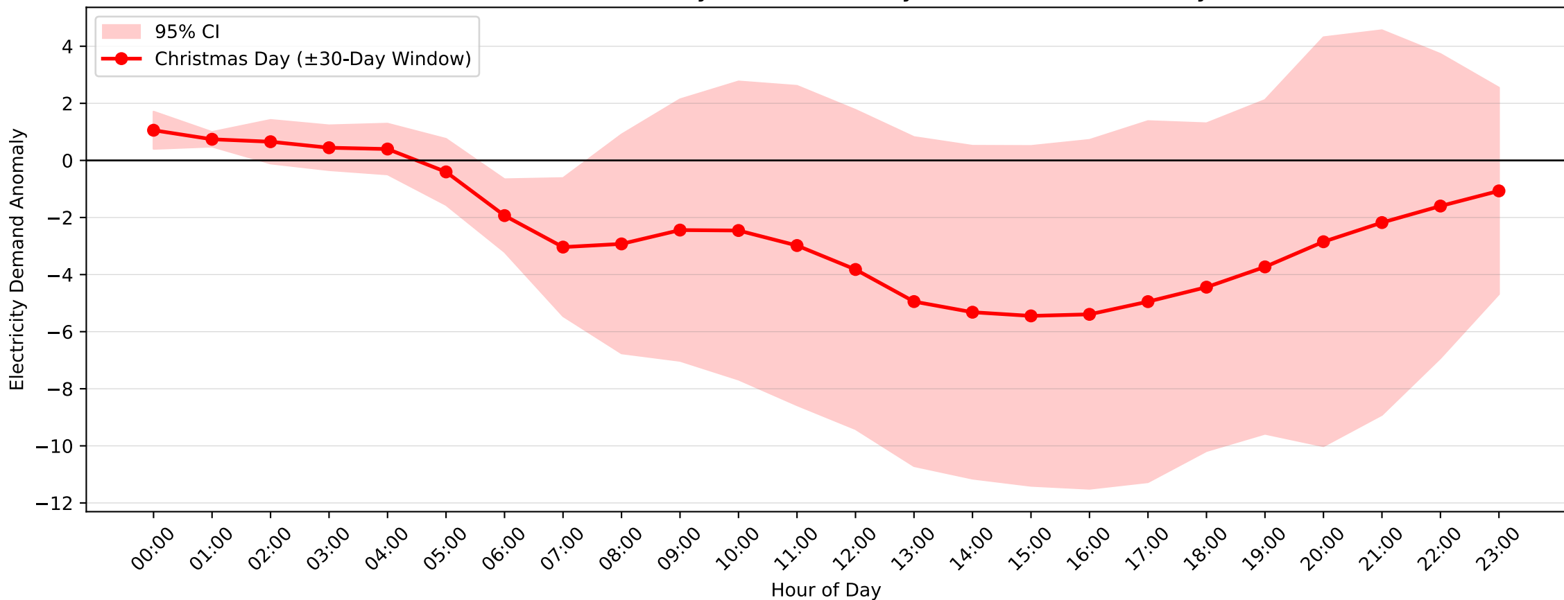
Hunters Hill Demand Anomaly: Christmas Day (2011-2012, \pm 30 -Day Window)
