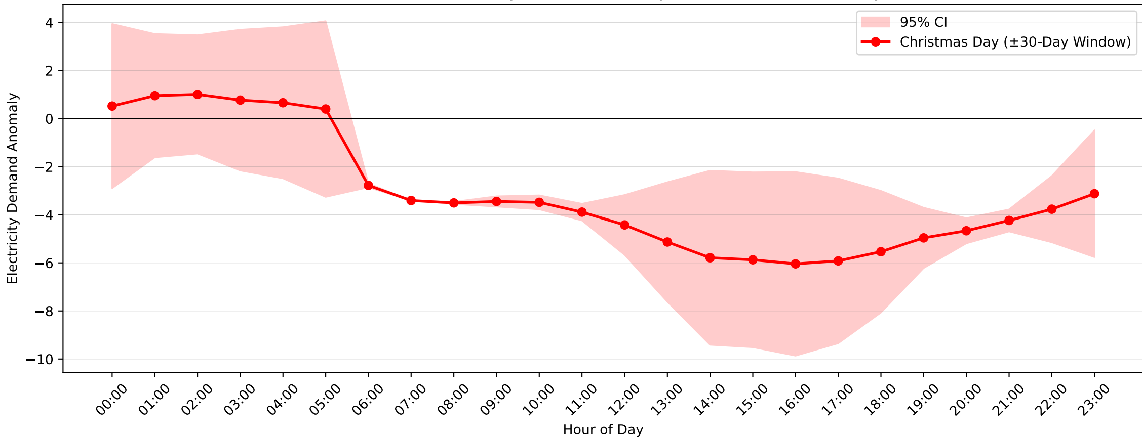
Hunters Hill Demand Anomaly: Christmas Day (2013-2014, \pm 30 -Day Window)
