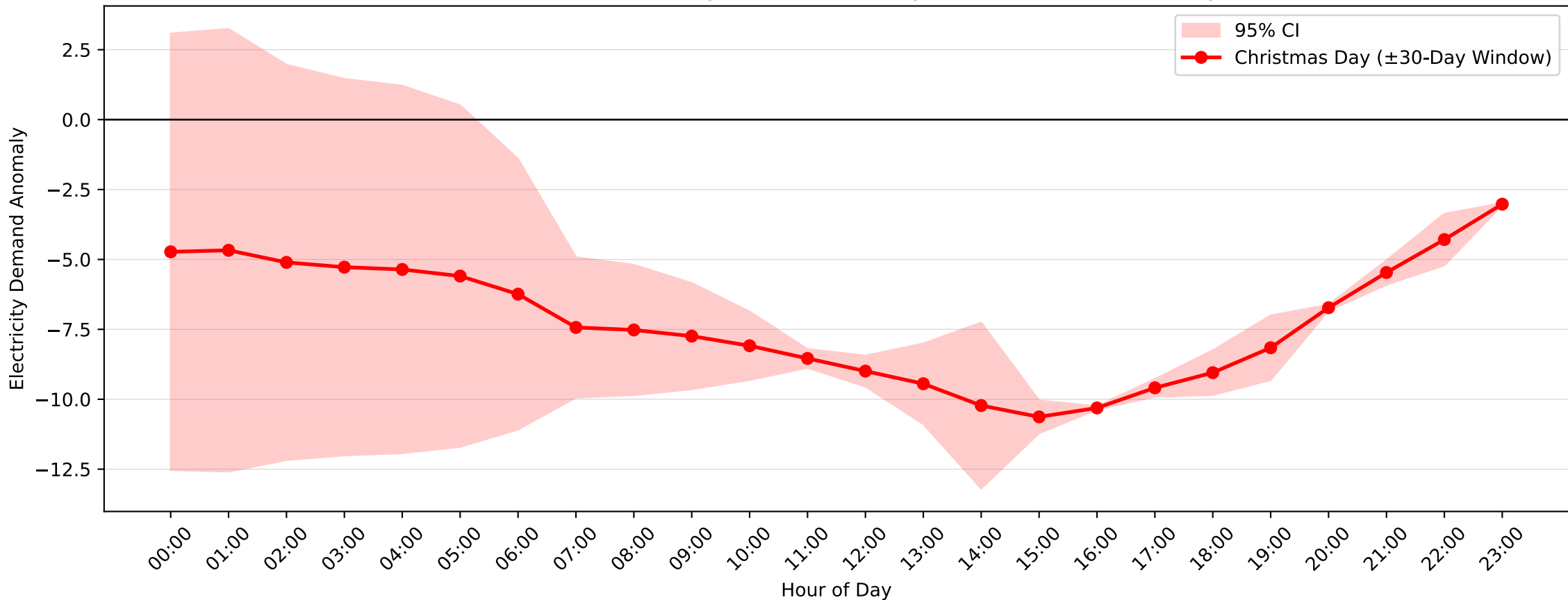
Hunters Hill Demand Anomaly: Christmas Day (2008–2009, \pm 30 -Day Window)
