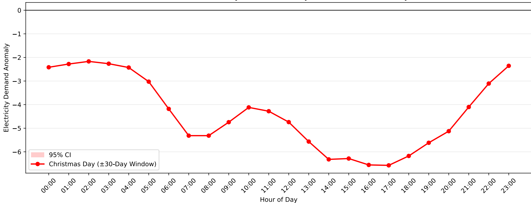
Hunters Hill Demand Anomaly: Christmas Day (2016–2017, \pm 30 -Day Window)
