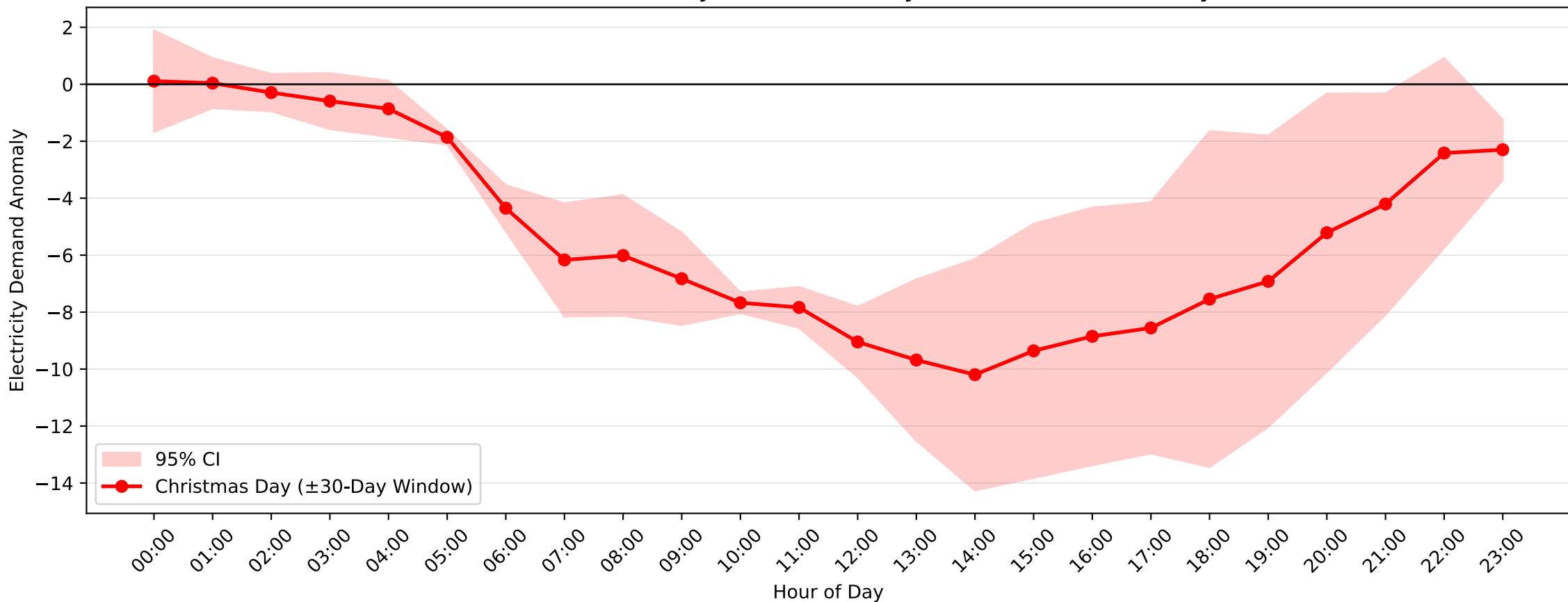
Hunters Hill Demand Anomaly: Christmas Day (2005-2006, \pm 30 -Day Window)
