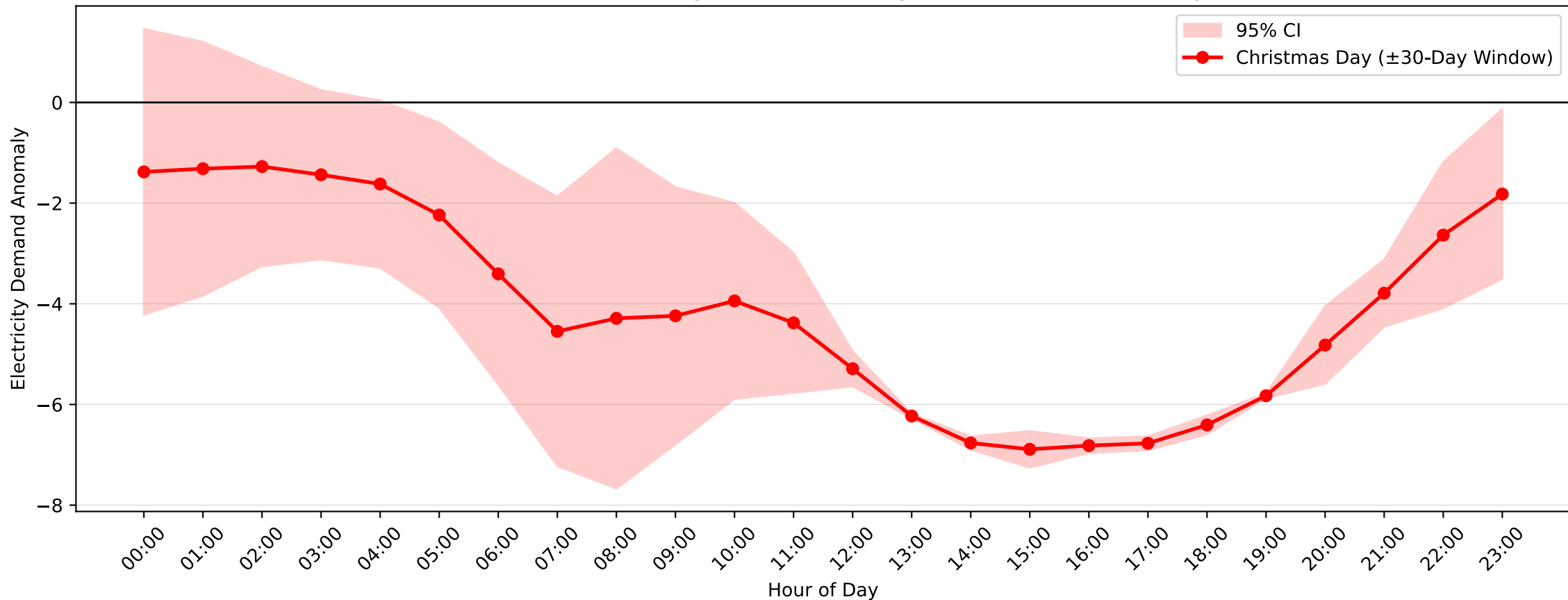
Hunters Hill Demand Anomaly: Christmas Day (2015–2016, \pm 30 -Day Window)
